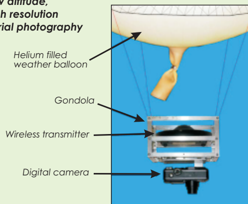
A side view of the high-resolution aerial photography rig designed by LEME's Andrew Baker.
